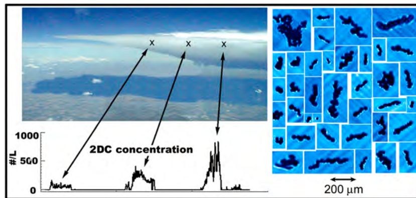
Figure 8. Photograph showing location of penetrations by the SPEC Learjet of an electrified midlatitude continental anvil at 39,000 ft msl ( T = -48^{\circ}\text{C} ) on 8 June 2001, time series of 2DC particle concentration and examples of CPI images.
