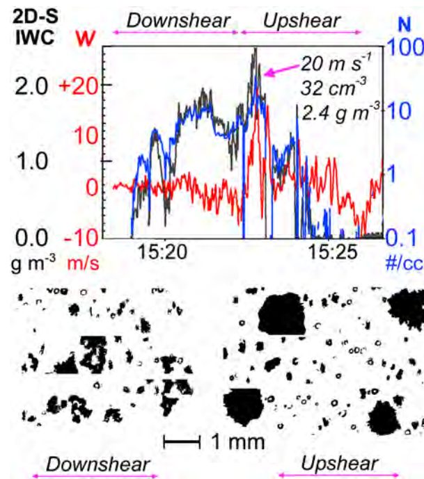
Figure 2. (top) Time series of ice water content (IWC), vertical air velocity ( w ), and particle concentration ( N ) from a DC-8 penetration at -47^{\circ}\text{C} of an embedded turret and (bottom) examples of 2D-S images. Data collected on 24 July 2007 during the TC4 project (from Lawson et al., 2010).
